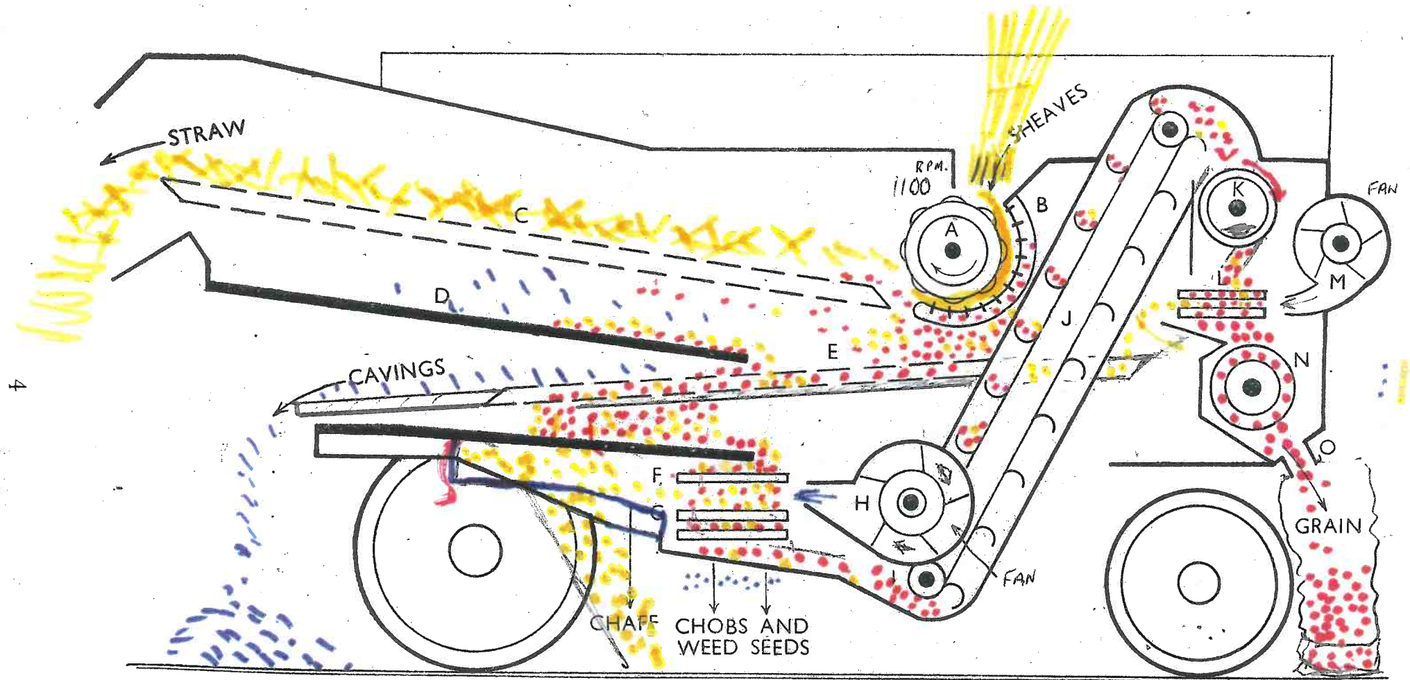
2. LONGITUDINAL SECTION THROUGH THRESHING MACHINE
